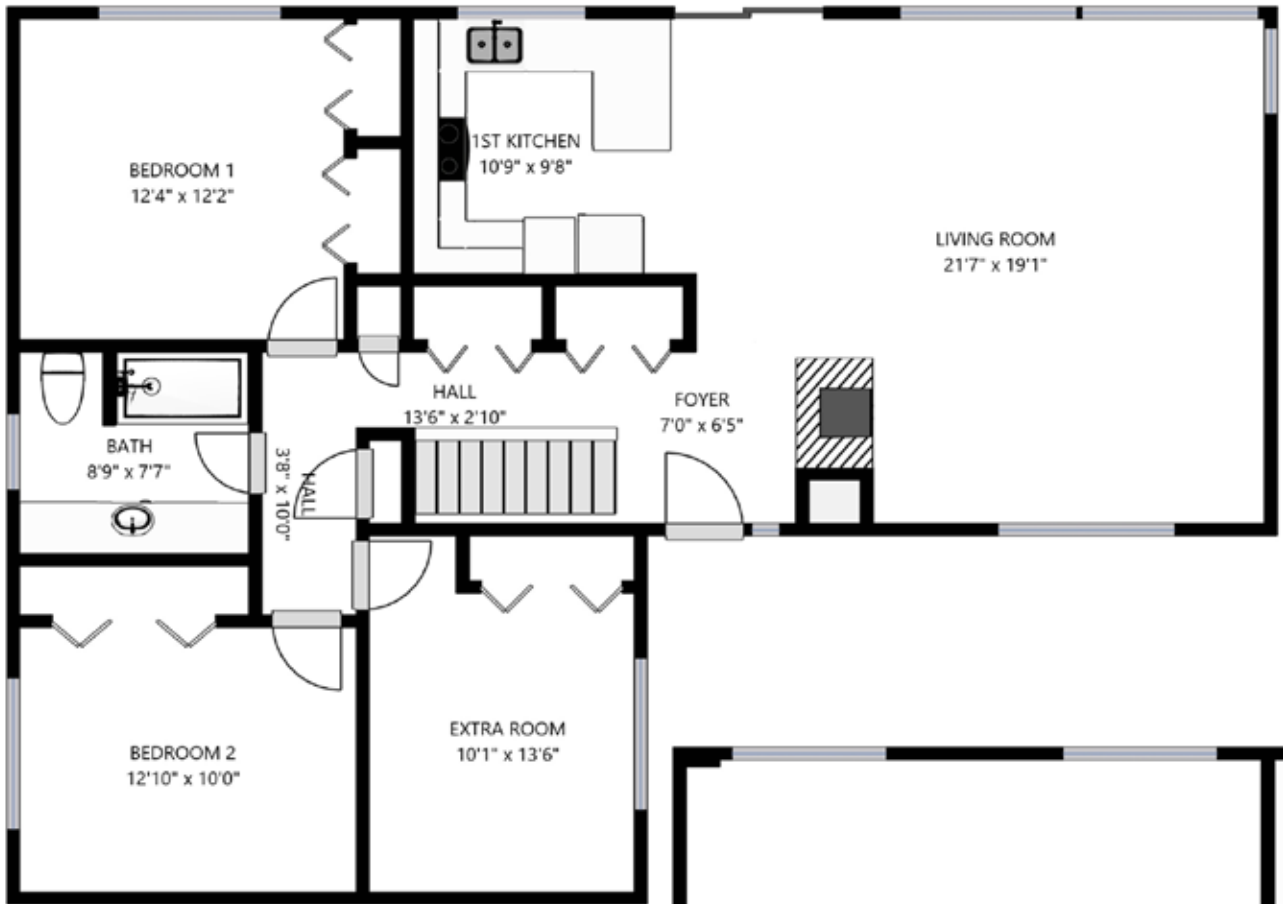
Main Floor
